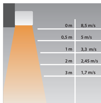
Distance/air speed
